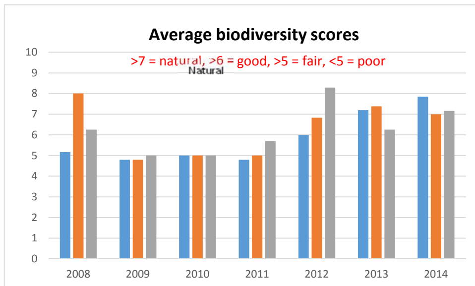
Figure 5: Mini-SASS average scores of last five years of river health monitoring at three sites on Mafinji River
